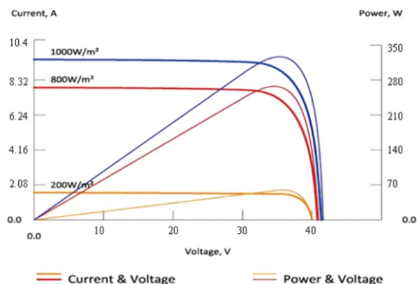
Current-Voltage & Power-Voltage characteristics various irradiance levels
